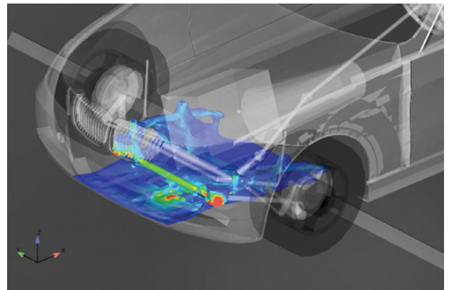
Figure 8. BMW Car Co-animation picture of Pole Run Over done by Adams & Marc and visualized in CEI Ensight
