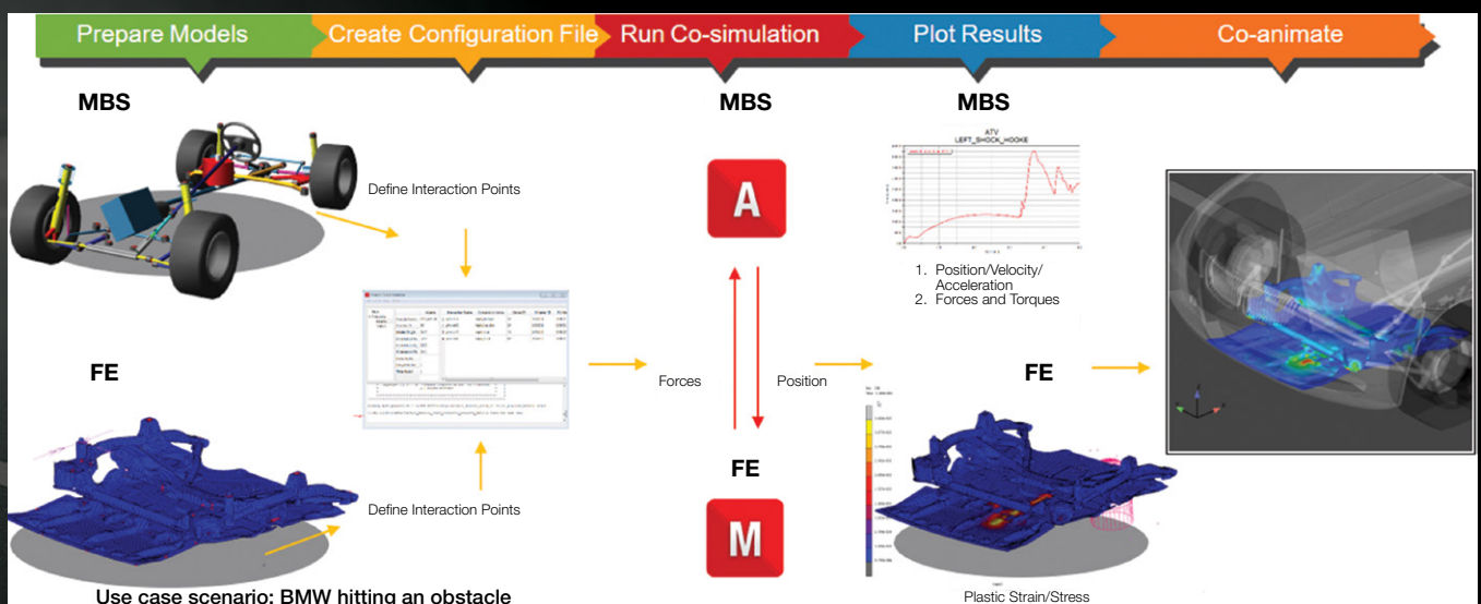
Figure 2. Typical Adams-Marc Co-Simulation Automotive Toolchain Workflow
